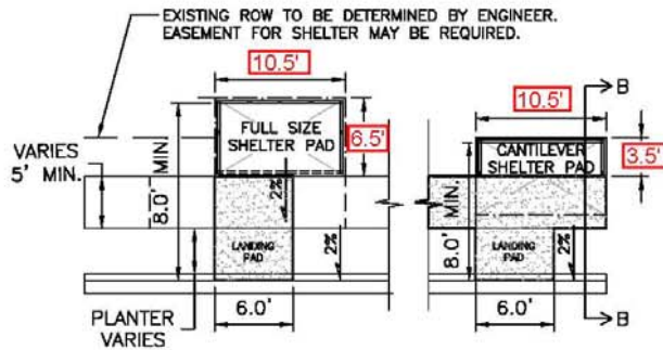
SHELTER BEHIND SIDEWALK W/PLANTER STRIP
