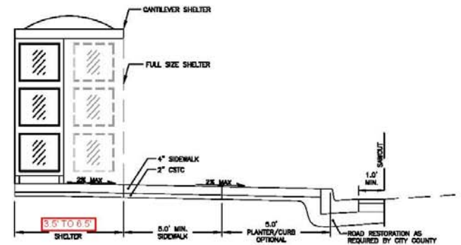
SECTION B-B SHELTER BEHIND SIDEWALK
