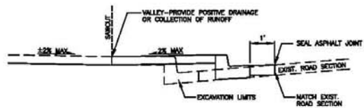
BULBOUT SECTION A-A 1"=20'
