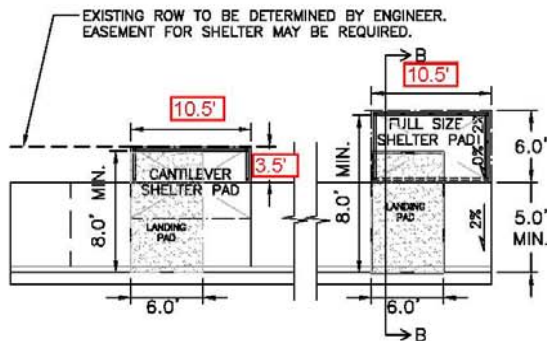
SHELTER BEHIND SIDEWALK
