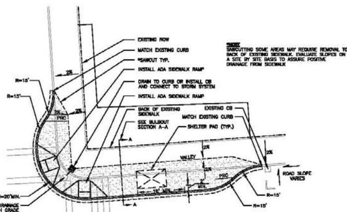
NEAR SIDE BULBOUT EXAMPLE 1"=10'
