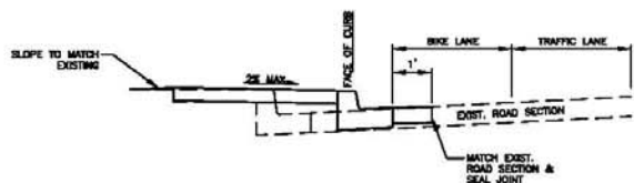
BULBOUT SECTION B-B 1"=20'
