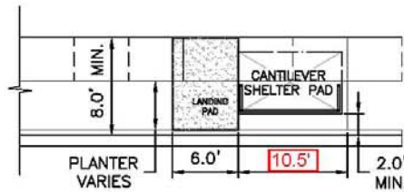
SHELTER IN PLANTER STRIP
