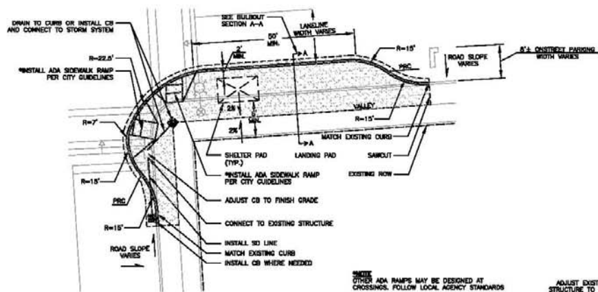
FAR SIDE BULBOUT EXAMPLE 1"=10'
