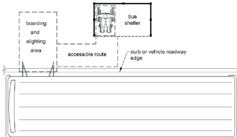
Figure 810.3 Bus Shelters
