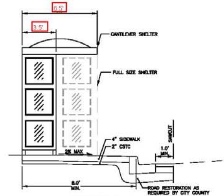
SECTION A-A SHELTER ON SIDEWALK
