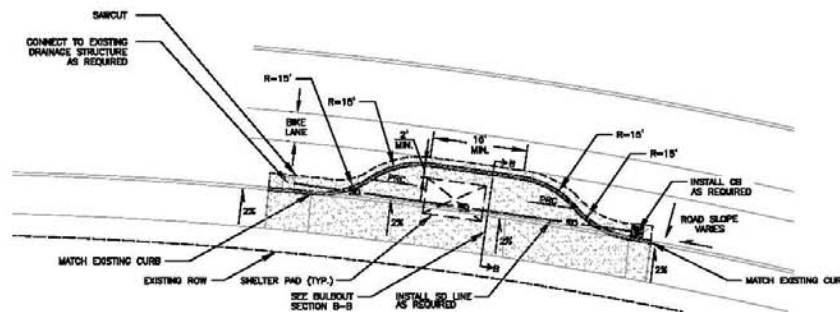
MID BLOCK BULBOUT STOP EXAMPLE 1"=10'
